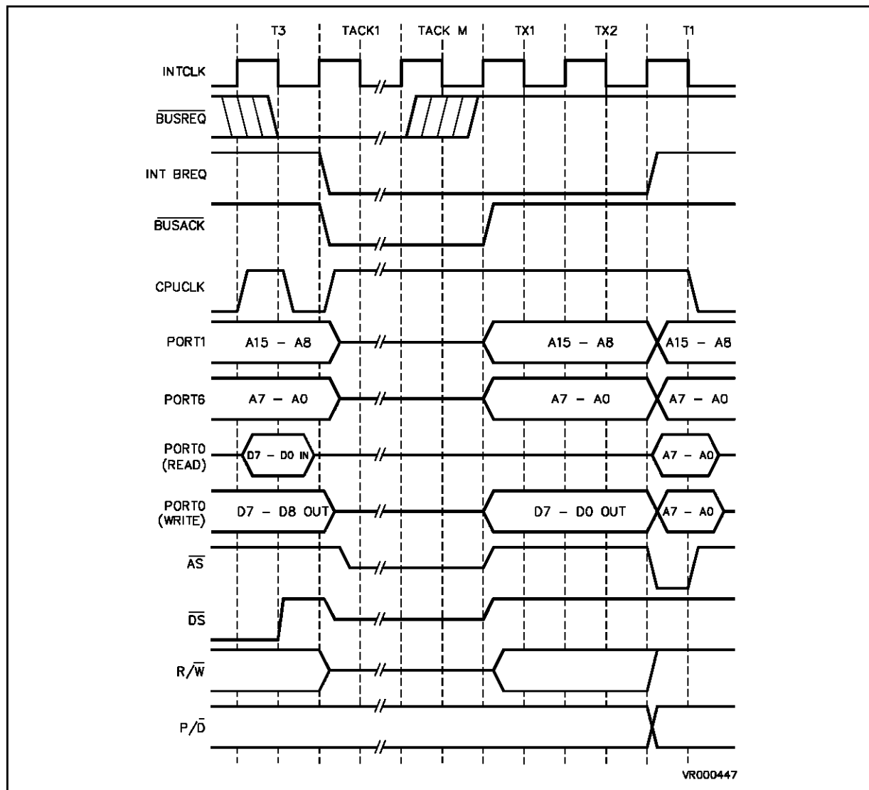
Figure 8-5. Bus Request/Acknowledge Timing.
