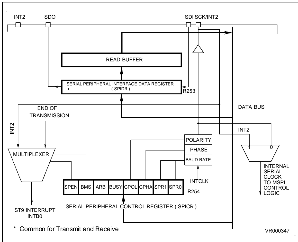
Figure 11-1. Block Diagram
