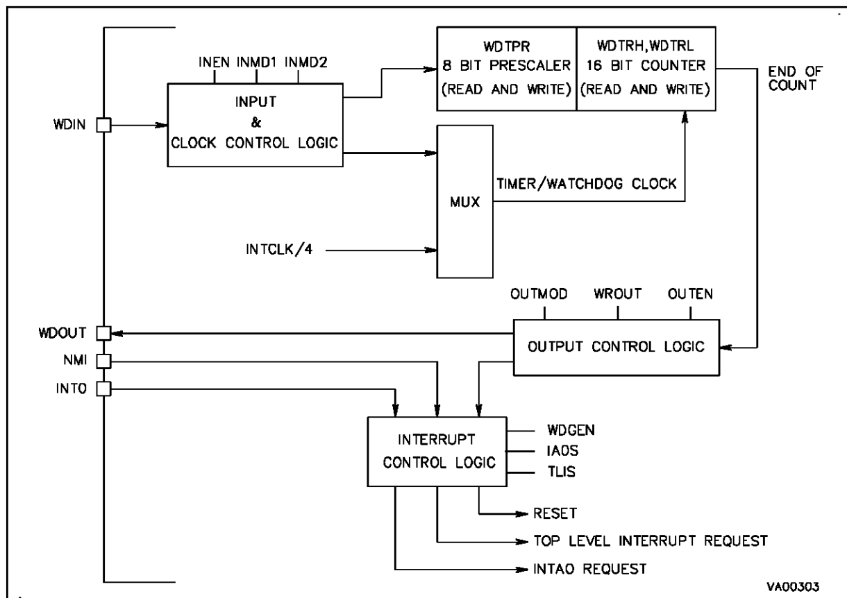
Figure 12-1. Block Diagram
