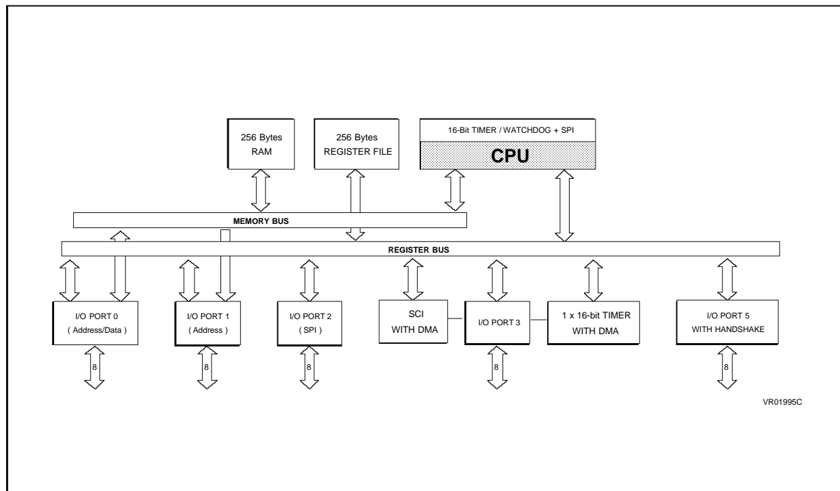
Figure 17-2. Block Diagram
