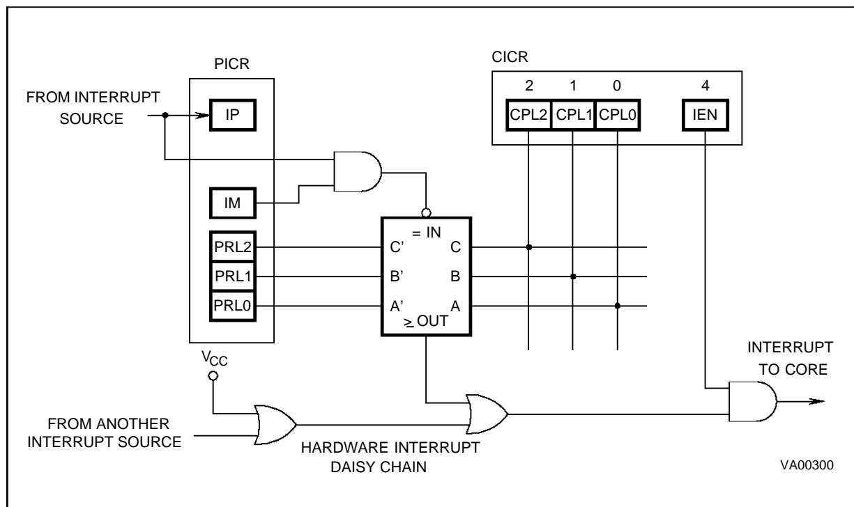
Figure 4-4. Interrupt Logic
