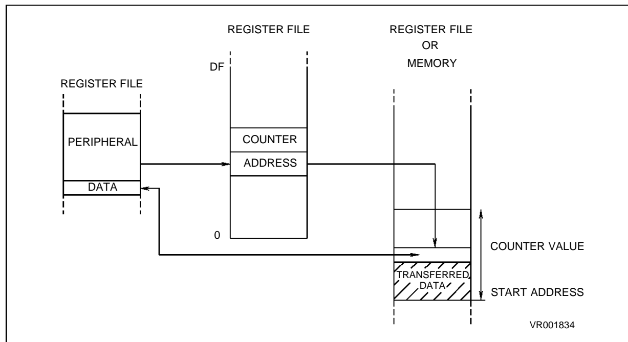
Figure 5-1. DMA Overview
