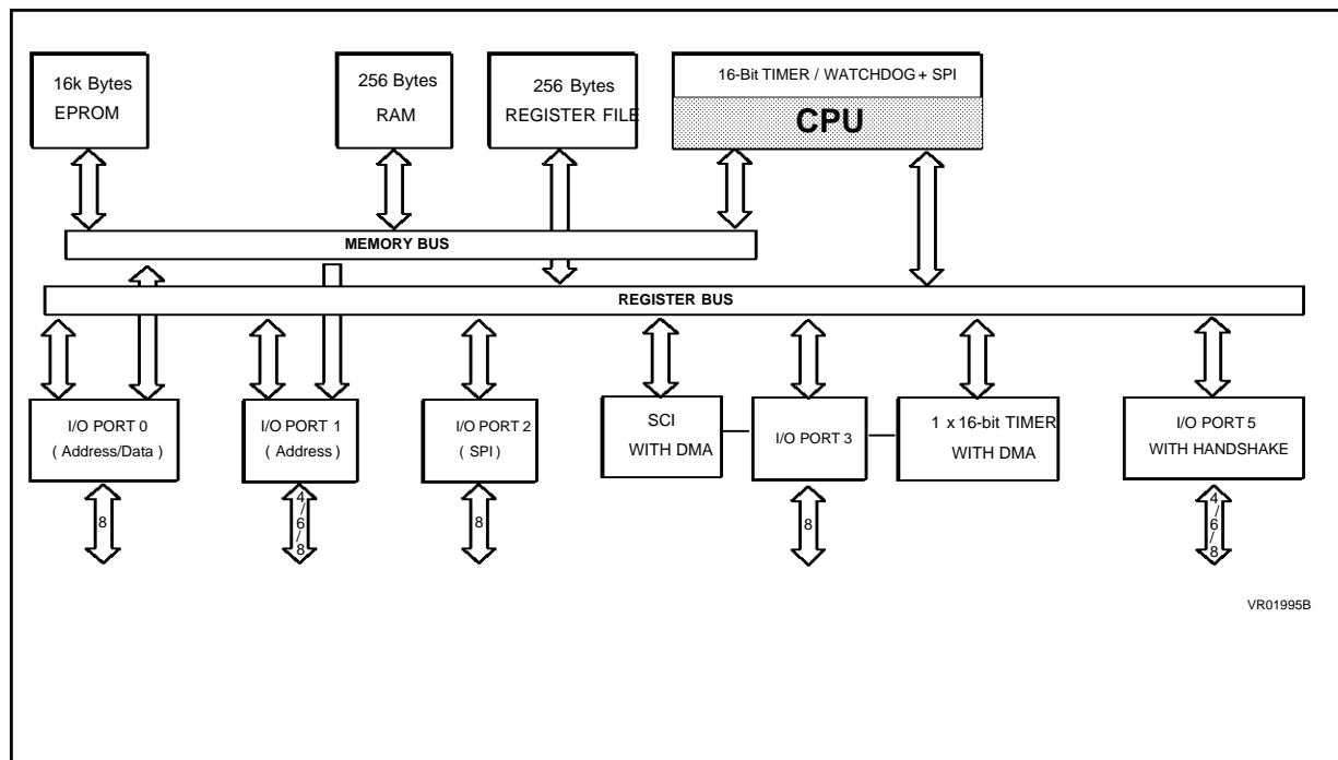
Figure 16-4. ST90E27, E28 Block Diagram
