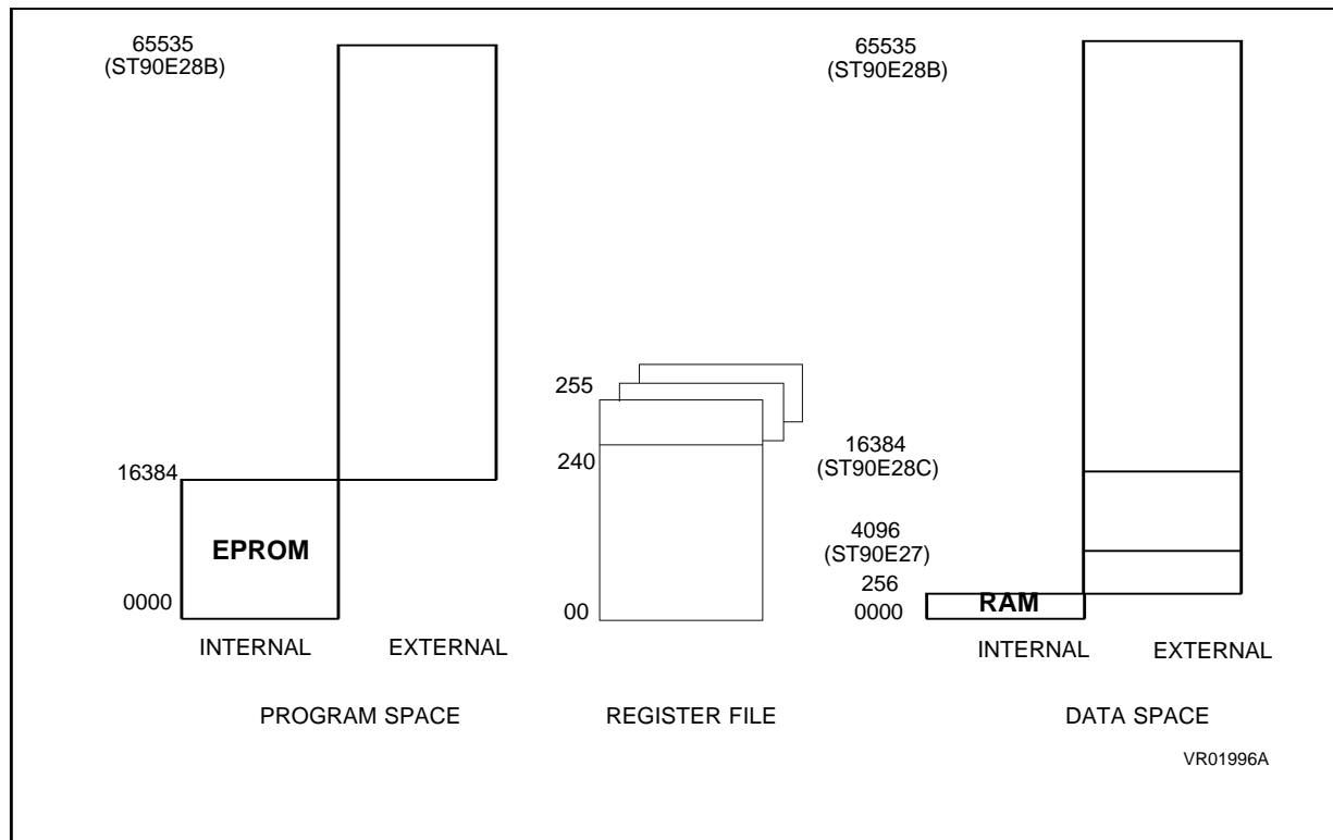
Figure 16-5. Memory Spaces
