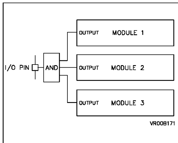
Figure 9-9. Example of 3 Alternate Function Outputs
