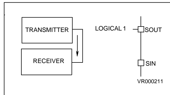
Figure 14-8. Loop Back Configuration
