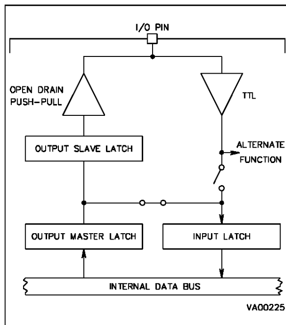
Figure 9-5. Output Configuration
