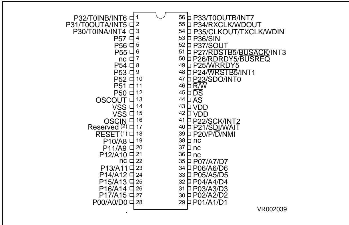
Figure 16-3. 56 Pin DIP Package
