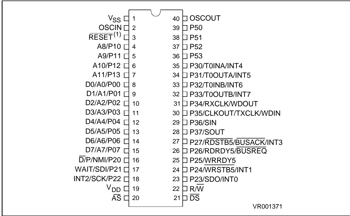
Figure 16-1. 40 Pin DIP Package
