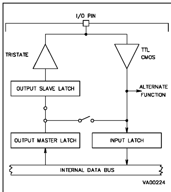
Figure 9-4. Input Configuration
