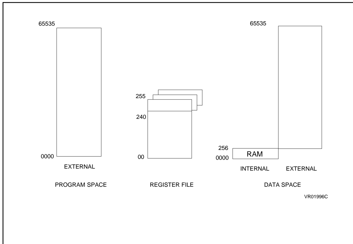
Figure 17-3. Memory Spaces
