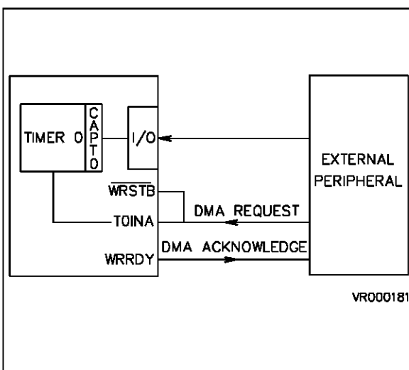
Figure 10-13. DMA with 2 Line Input Handshake Mode
