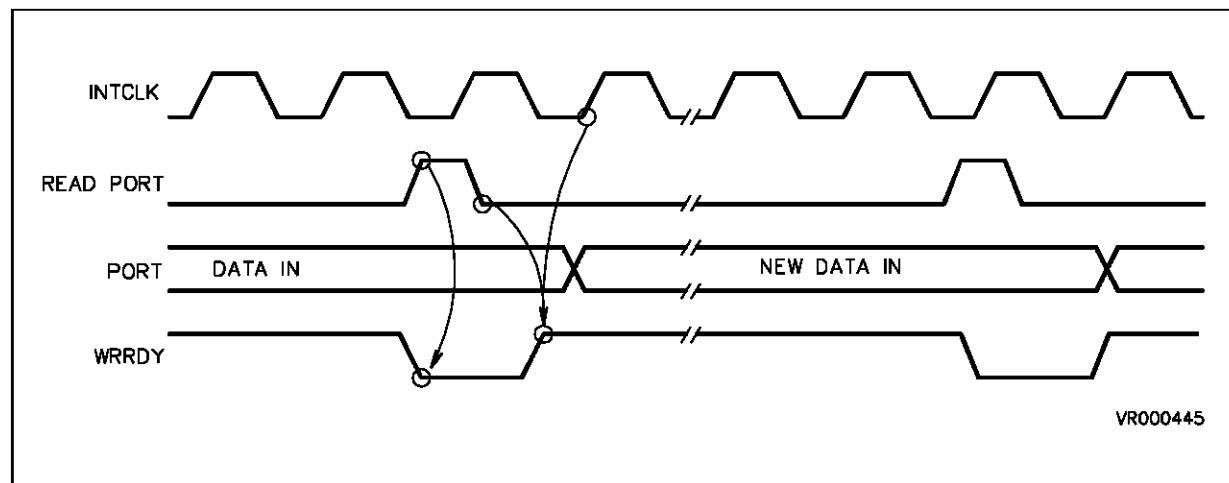
Figure 10-5. One Line Input Handshake Timing
