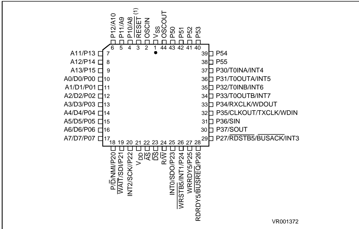
Figure 16-2. 44 Pin PLCC Package
