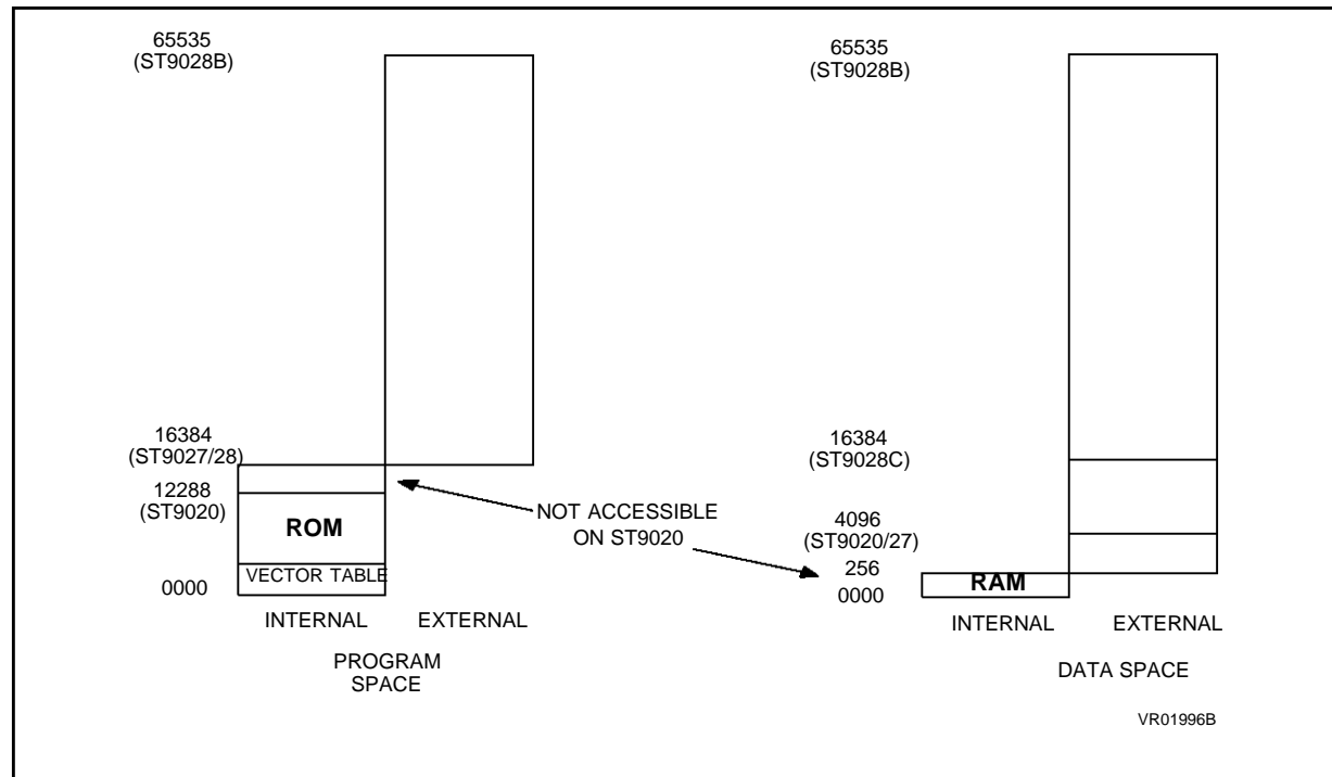
Figure 3-1. Memory Map
